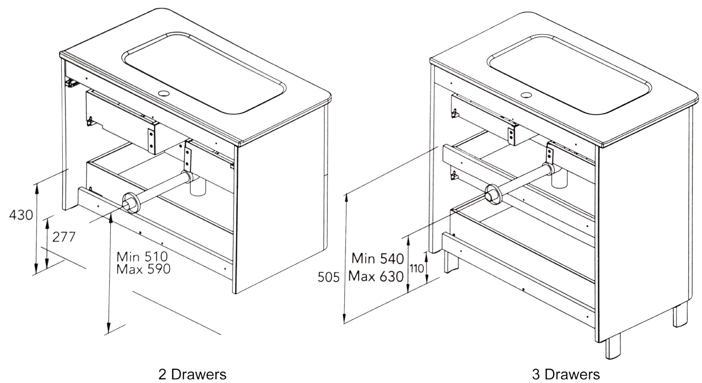
Placement Scheme For Syphon
