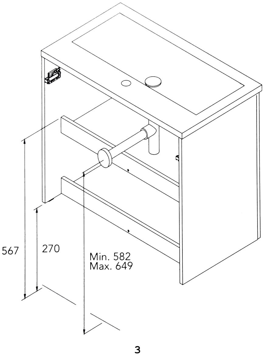
Placement Scheme For Syphon
